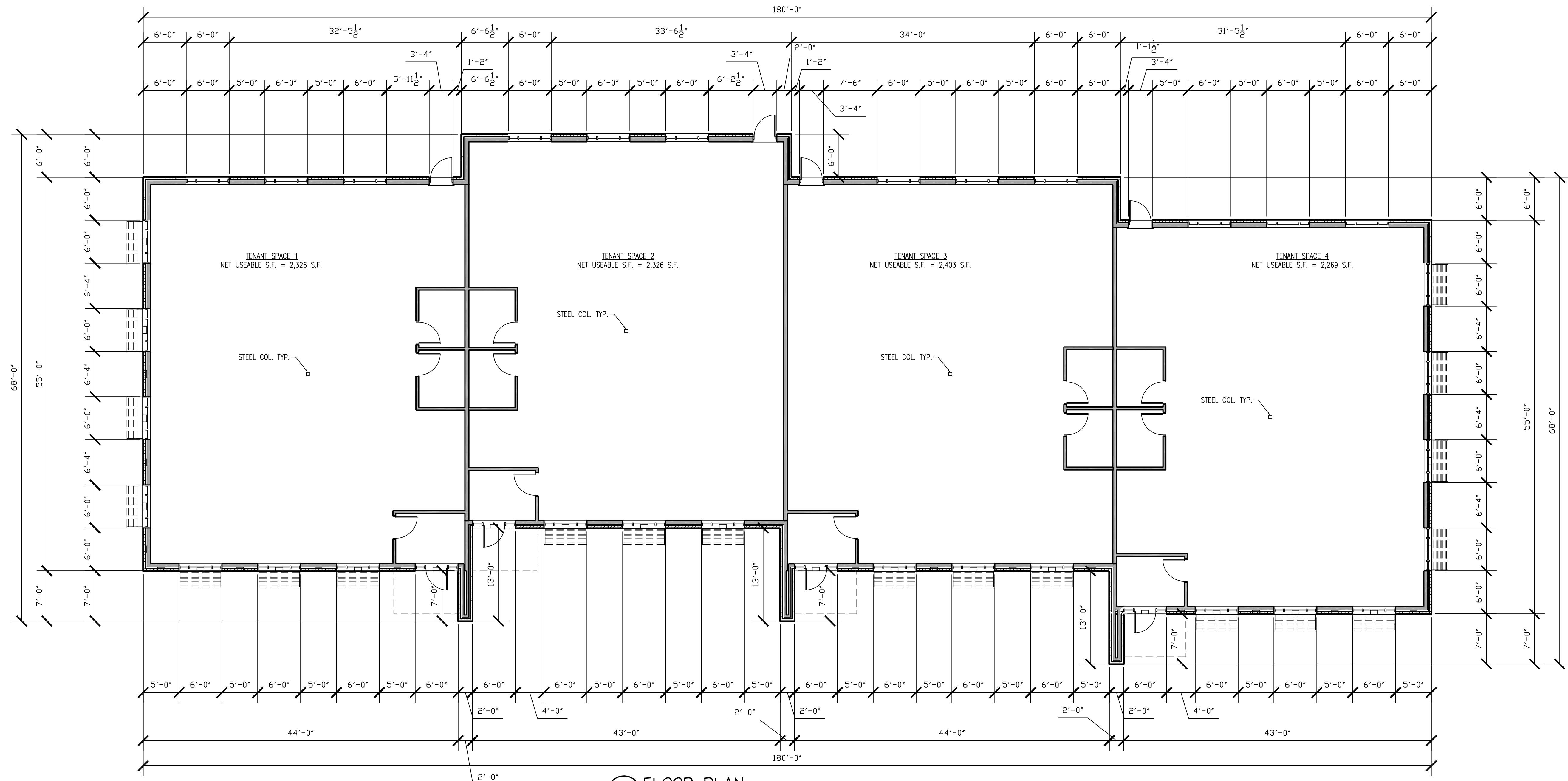
1 FLOOR PLAN SCALE: 1/8"=1'-0" BUILDING AREA: 9,963 S.F.
